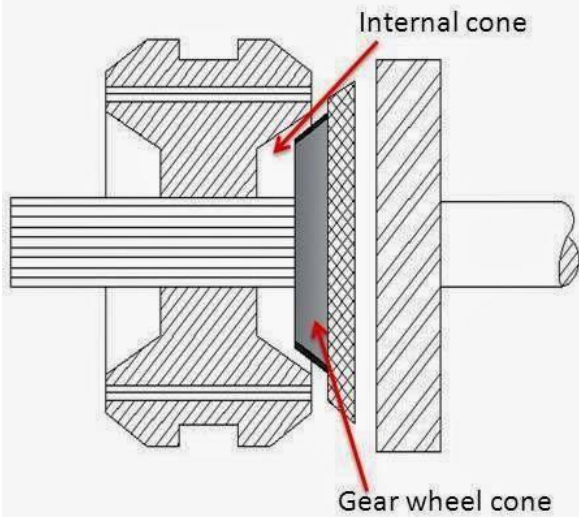
Synchromesh device in disengage position
